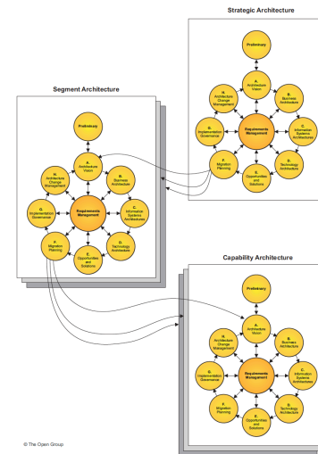
Figure 18-3 A Hierarchy of ADM Processes Example
